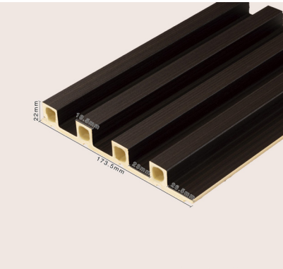
Name: 170 Grille Size: 173.5x2800x22mm One 20GP container can load 780 boxes
