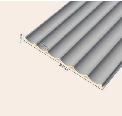
Name: 206 Corrugated board Size: 206x2800x15mm One 20GP container can load 352 boxes
