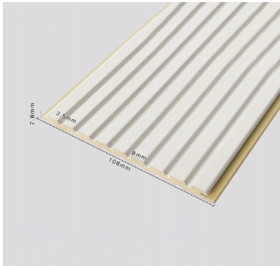
Name: 1039 Premium grille Size: 108x2800x7.8mm One 20GP container can load 784 boxes
