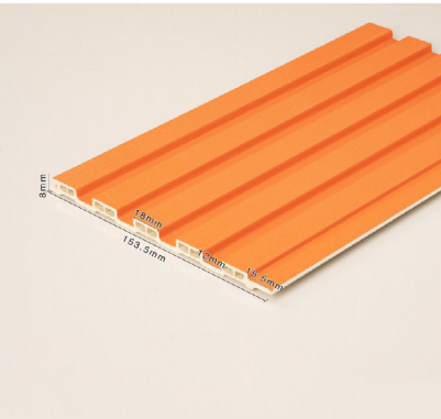
Name: 150 Little Great Wall Size: 173.5x2800x22mm One 20GP container can load 468 boxes
