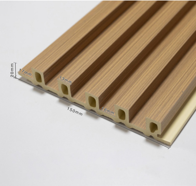
Name: 139 Grille Size: 150x2800x20mm One 20GP container can load 784 boxes
