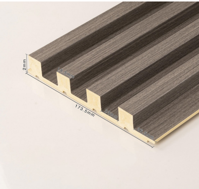
Name: 166 Solid grille Size: 173.5x2800x22mm One 20GP container can load 780 boxes
